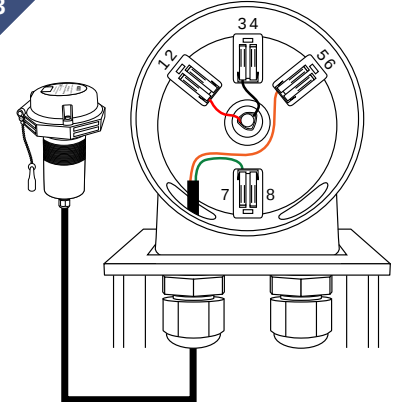
Uplink wire Connection to Junction Box Orange wire Terminal 5, Green wire Terminal 7
