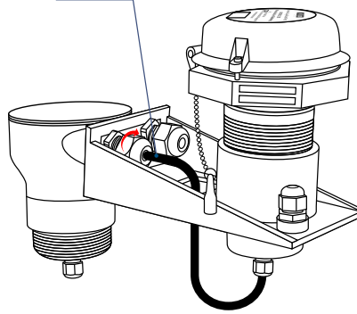
Uplink wire Connection to Junction Box Green & Orange Wires
